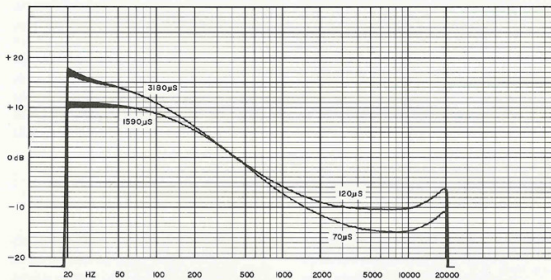
Figure 4 Frequency Response of Nakamichi 1000 Playback EQ. Amp.
