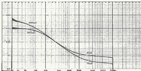
Figure 6 Frequency Response of Nakamichi 1000 EQ. Amp Specially Modified for Test Purposes.
