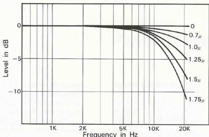
Figure 3 Head Gap Loss.
