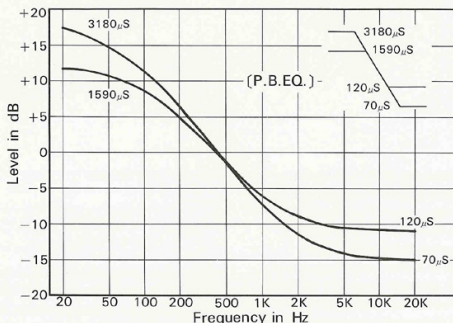
Figure 1 Theoretical Playback Equalization Curves.
