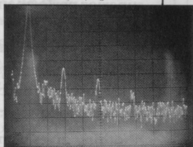
Distortion@100Hz@200nVb/m Horizontal 100Hz/div.; Vertical 10dB div. Start Frequency 0Hz
