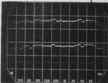
Pink Noise Frequency Response (Type IV) Log Sweep; Vertical 10dB/division Frequency as per graticule.
