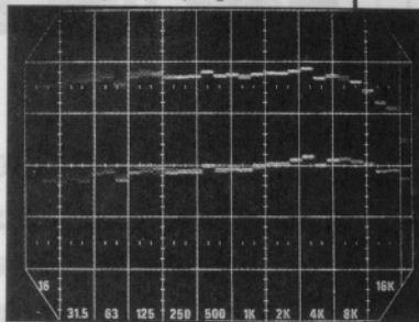
Pink Noise Frequency Response (Type II) Log Sweep; Vertical 10dB/division Frequency as per graticule.
