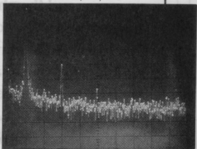
Distortion@1kHz@200nVb/m Horizontal 100Hz/div.; Vertical 10dB div. Start Frequency 0Hz
