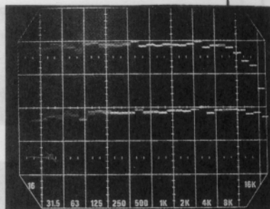
Pink Noise Frequency Response (Type I) Log Sweep; Vertical 10dB/division Frequency as per graticule.
